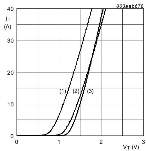
Fig. 10. On-state current as a function of on-state voltage V_o = 1.164 \text{ V}; R_s = 0.027 \Omega
