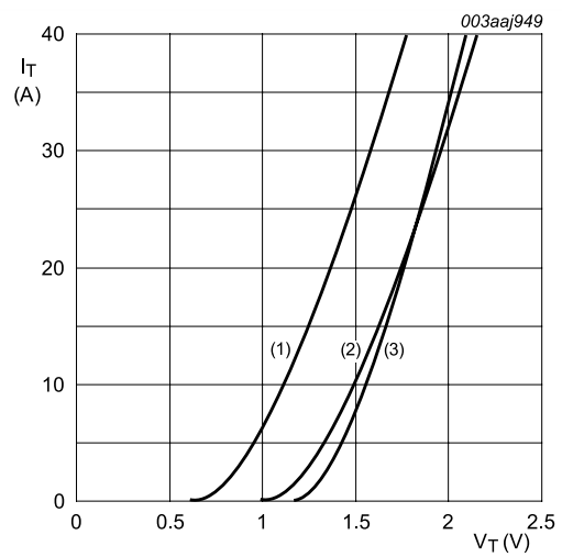
V_o = 1.145 V; R_s = 0.031 \Omega Fig. 10. On-state current as a function of on-state voltage
